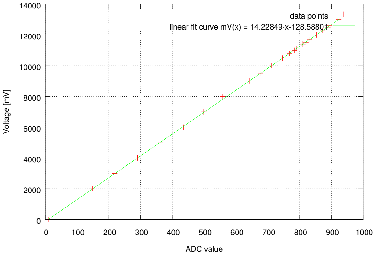
Voltage to measured ADC
